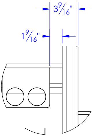
DETAIL B SCALE 1 : 7
